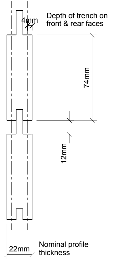
Interlocking Arrangement
